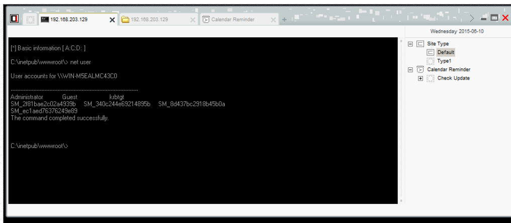
WebShell that Dllshellexc2010 provides inside the China Chopper graphical user interface (GUI)
