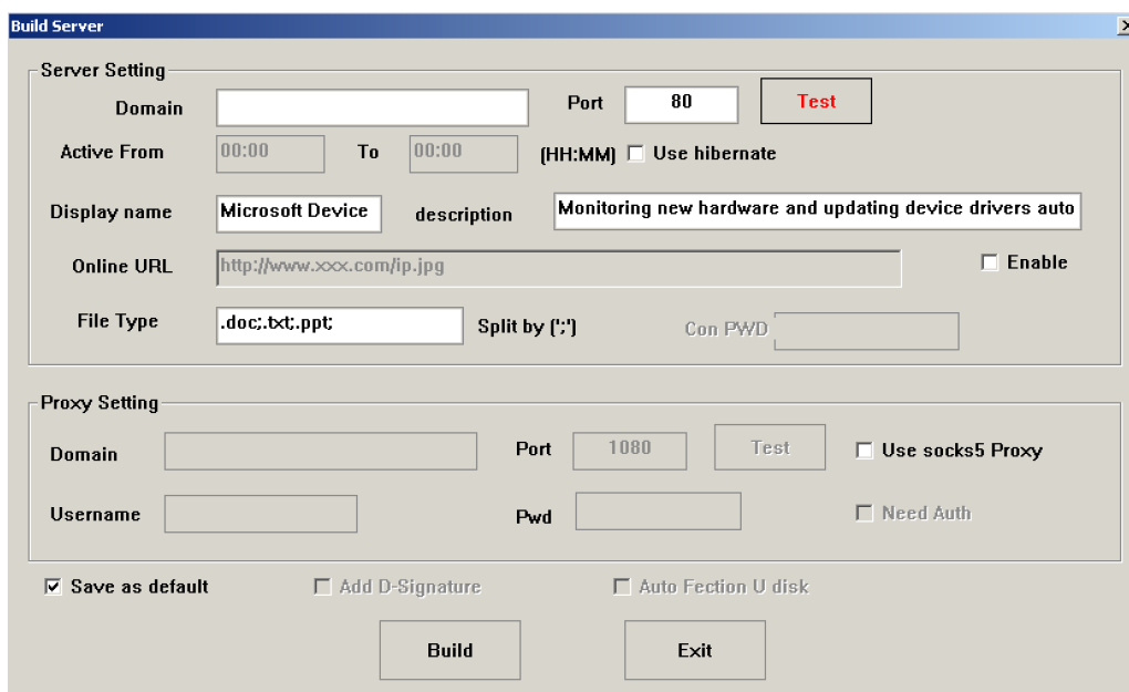
Ring RAT's Build Server features
