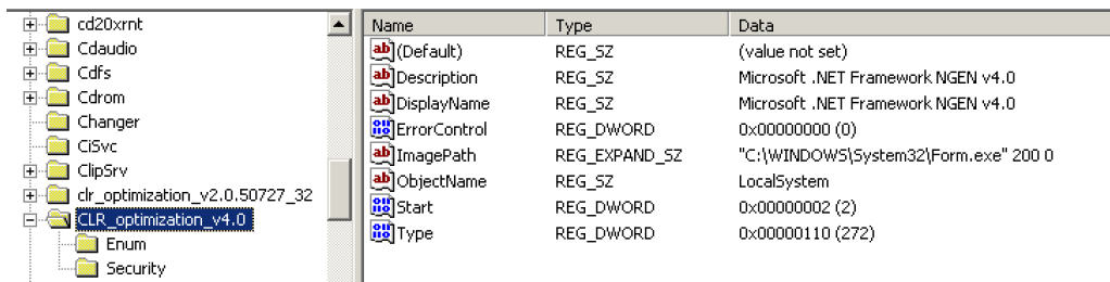
PlugX infection as seen in the Windows registry
