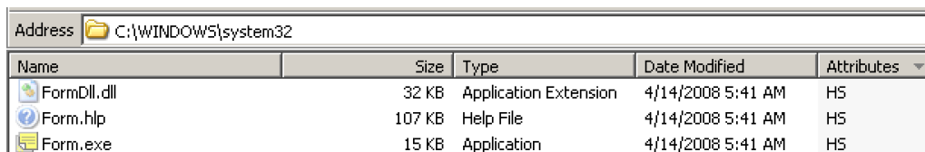
PlugX files hidden in system32
