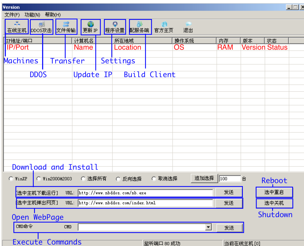
NBDDOS controller's GUI
