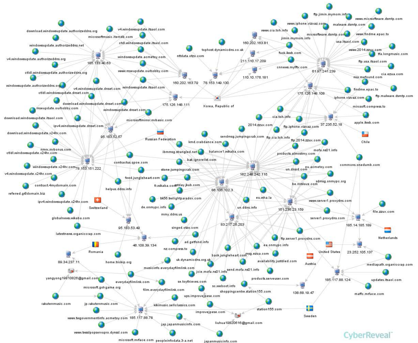
Figure 8: High-level view of infrastructure used by APT10 throughout 2016
