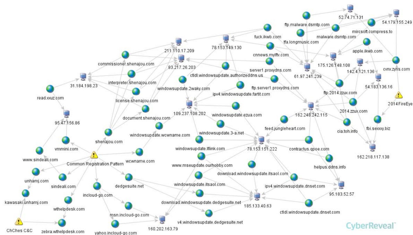
Figure 11: Infrastructure graph linking early PlugX domains to recent ChChes domains
