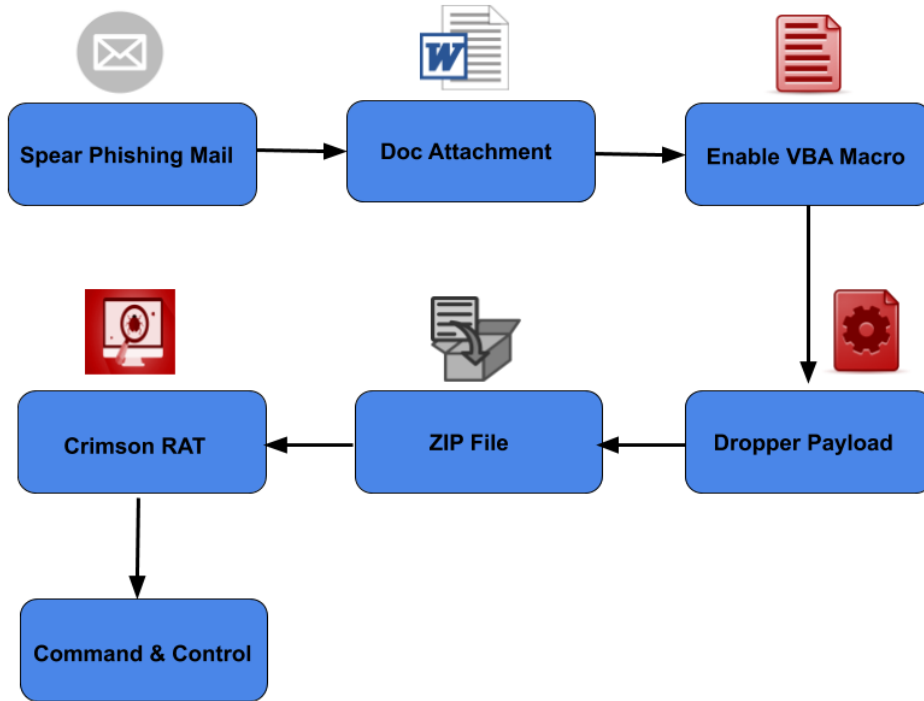
Image: Infection Chain – Scenario 1
