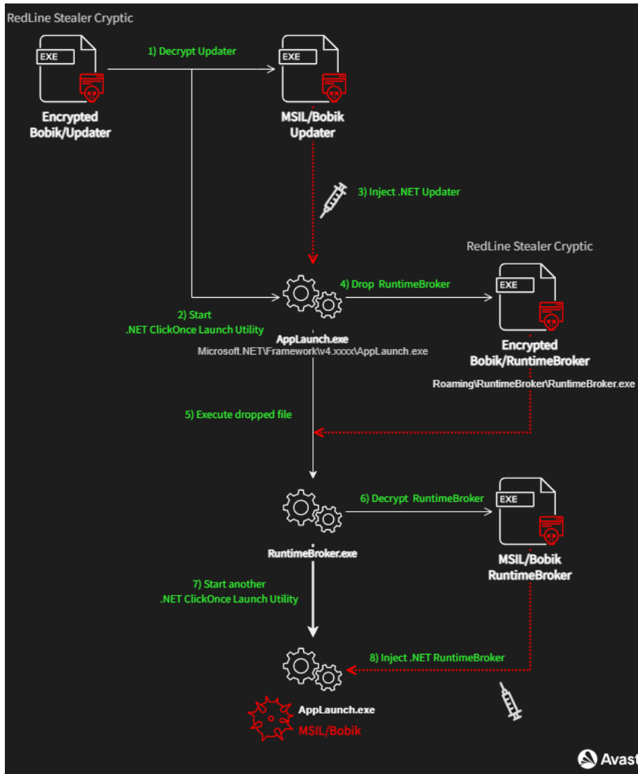
Bobik deployment using RedLine Stealer Cryptic
