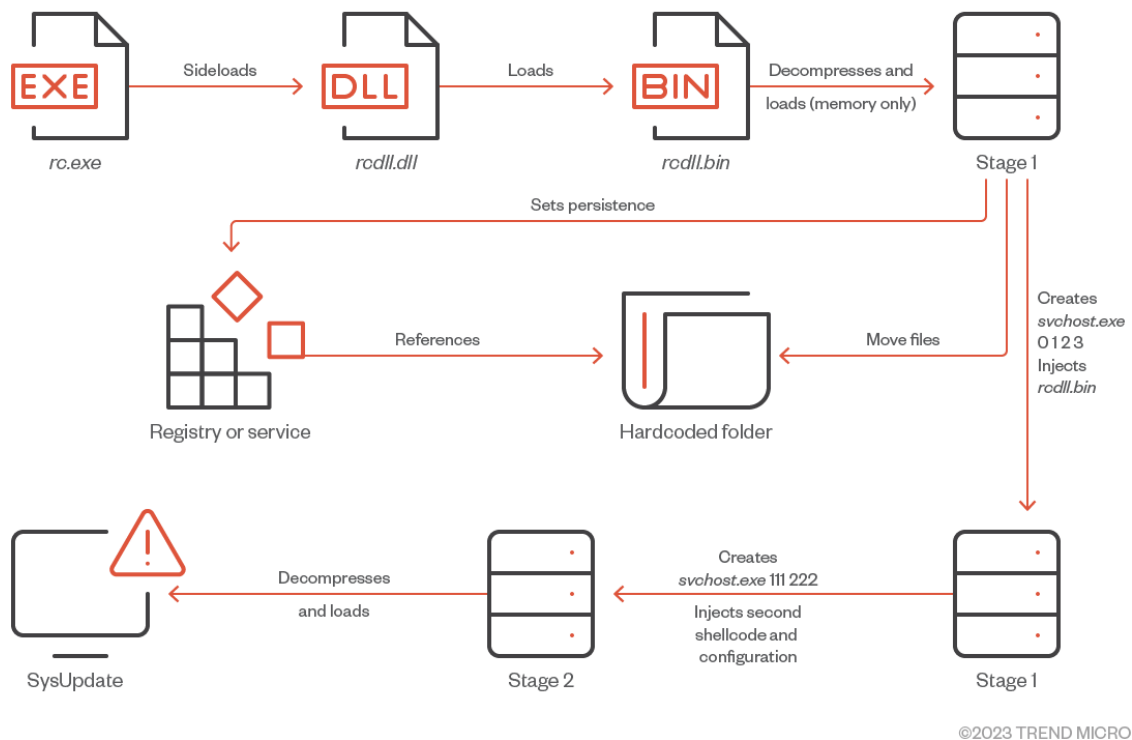
Figure 1. Updated SysUpdate loading process routine
