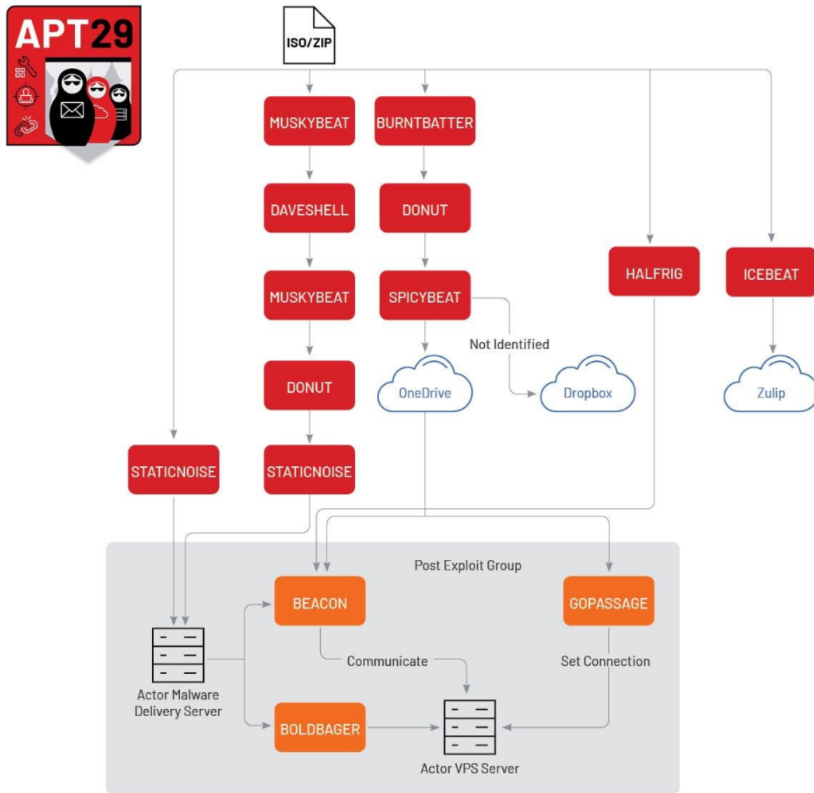
Figure 10: APT29's Second-Stage Downloaders Used in 2023
