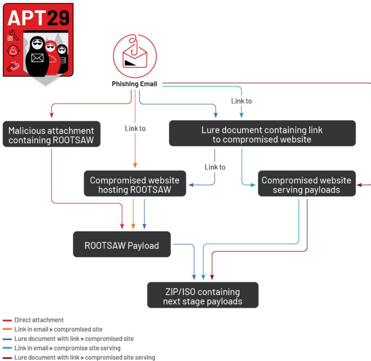
Figure 2: APT29's diverse first-stage delivery methods
