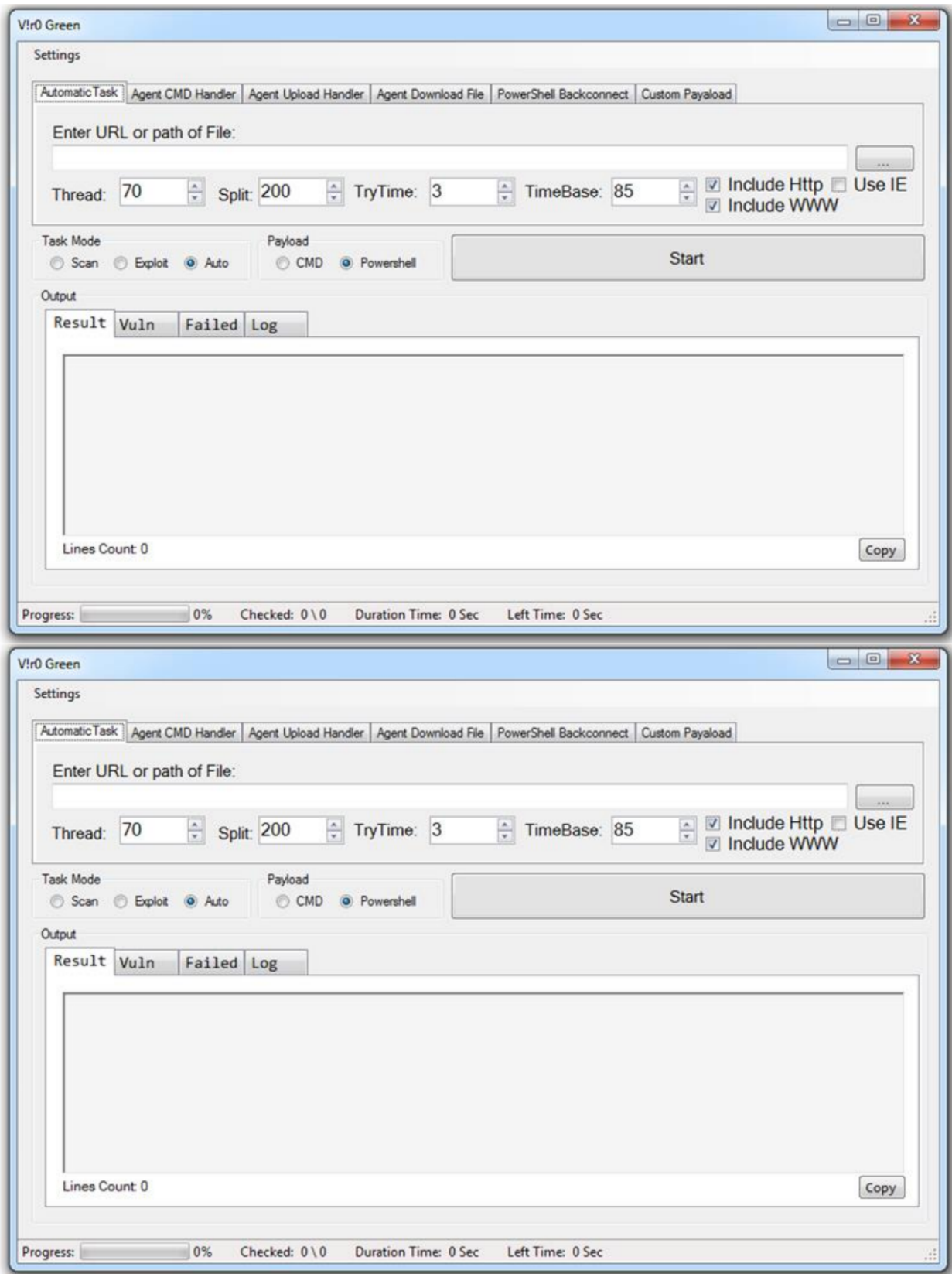
Figure 7: VIROGREEN GUI
