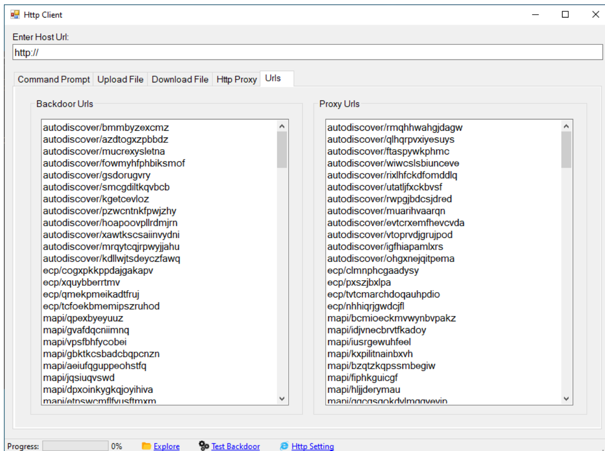
Figure 6: URLs Tab
