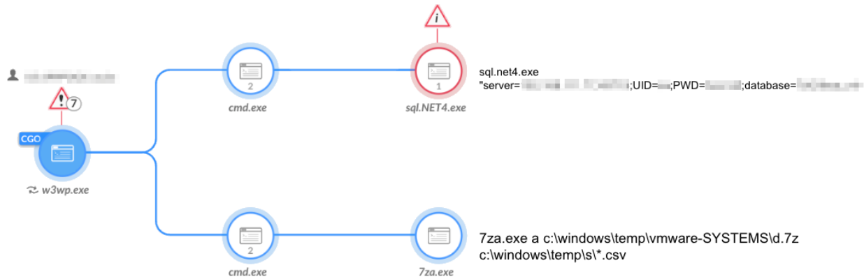
Figure 10. Sql extractor and 7za.exe used to extract files and archive them.
