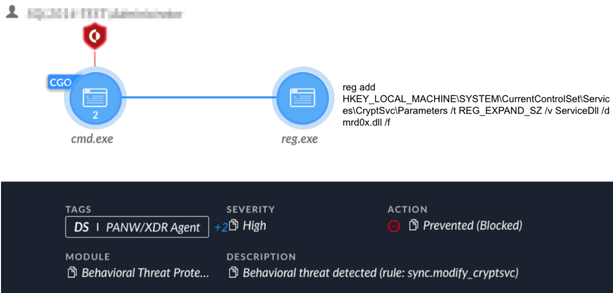
Figure 37. Cortex XDR prevents service registry manipulation.
