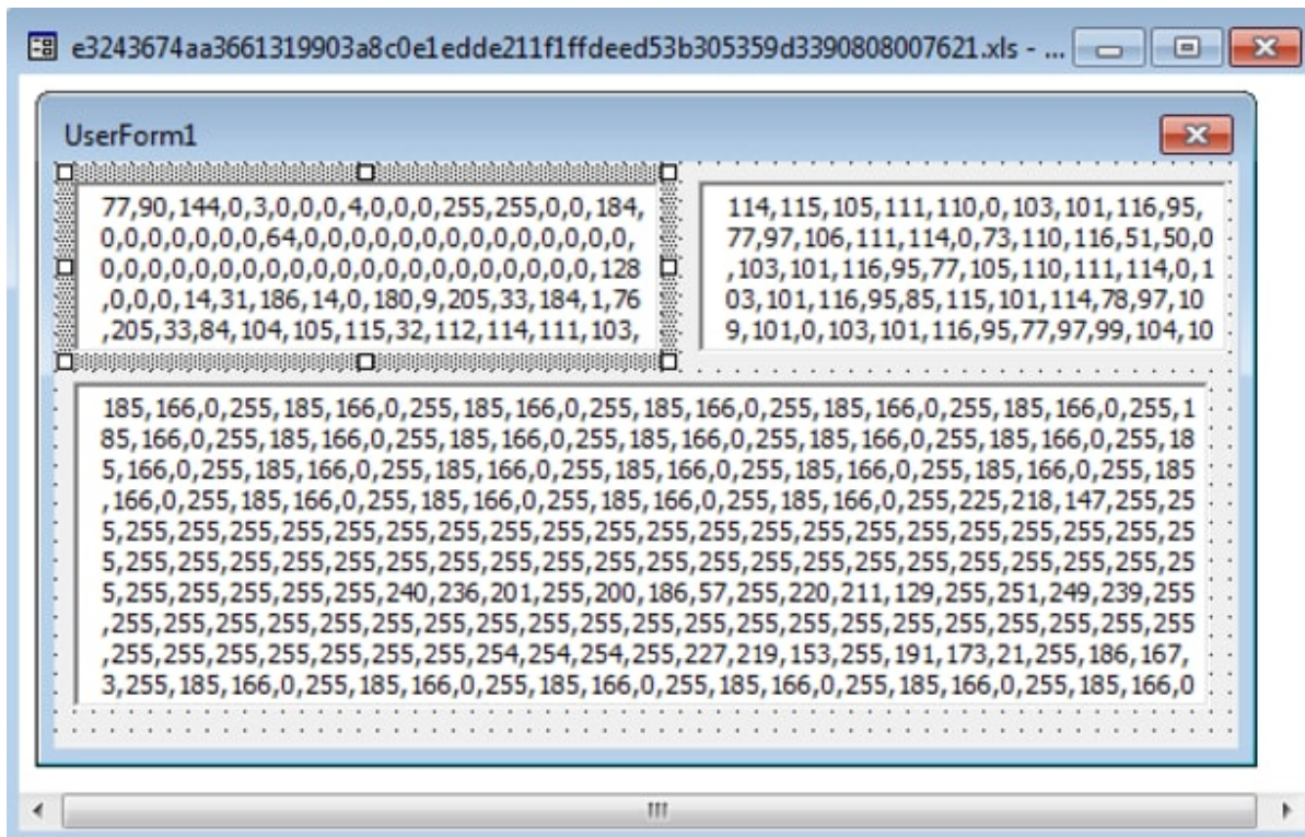
Figure 13 Embedded user form with three text boxes
