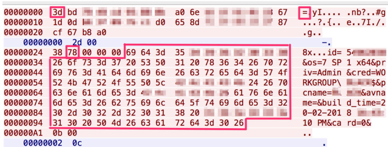
Figure 7: Screenshot of FlawedAmmyy C&C protocol from Wireshark
