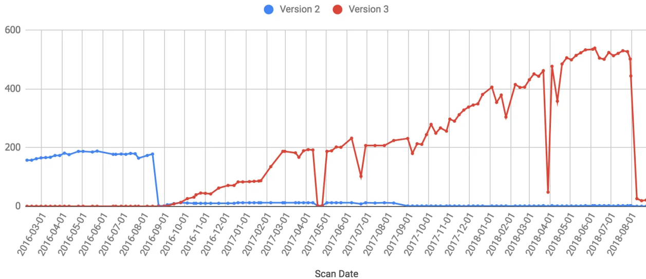
Figure 4: Pegasus servers available over time.
