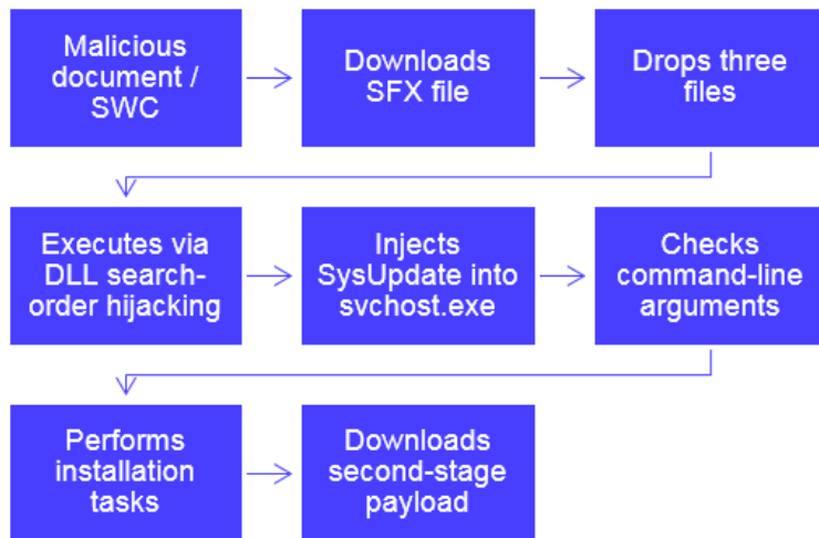
Figure 6. SysUpdate stage 1 installation process. (Source: Secureworks)
