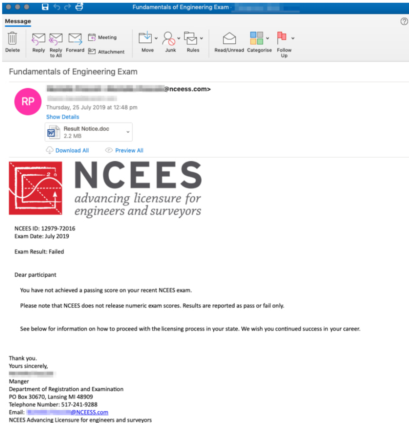
Figure 4 NCEES-themed phishing email delivering LookBack malware July 2019
