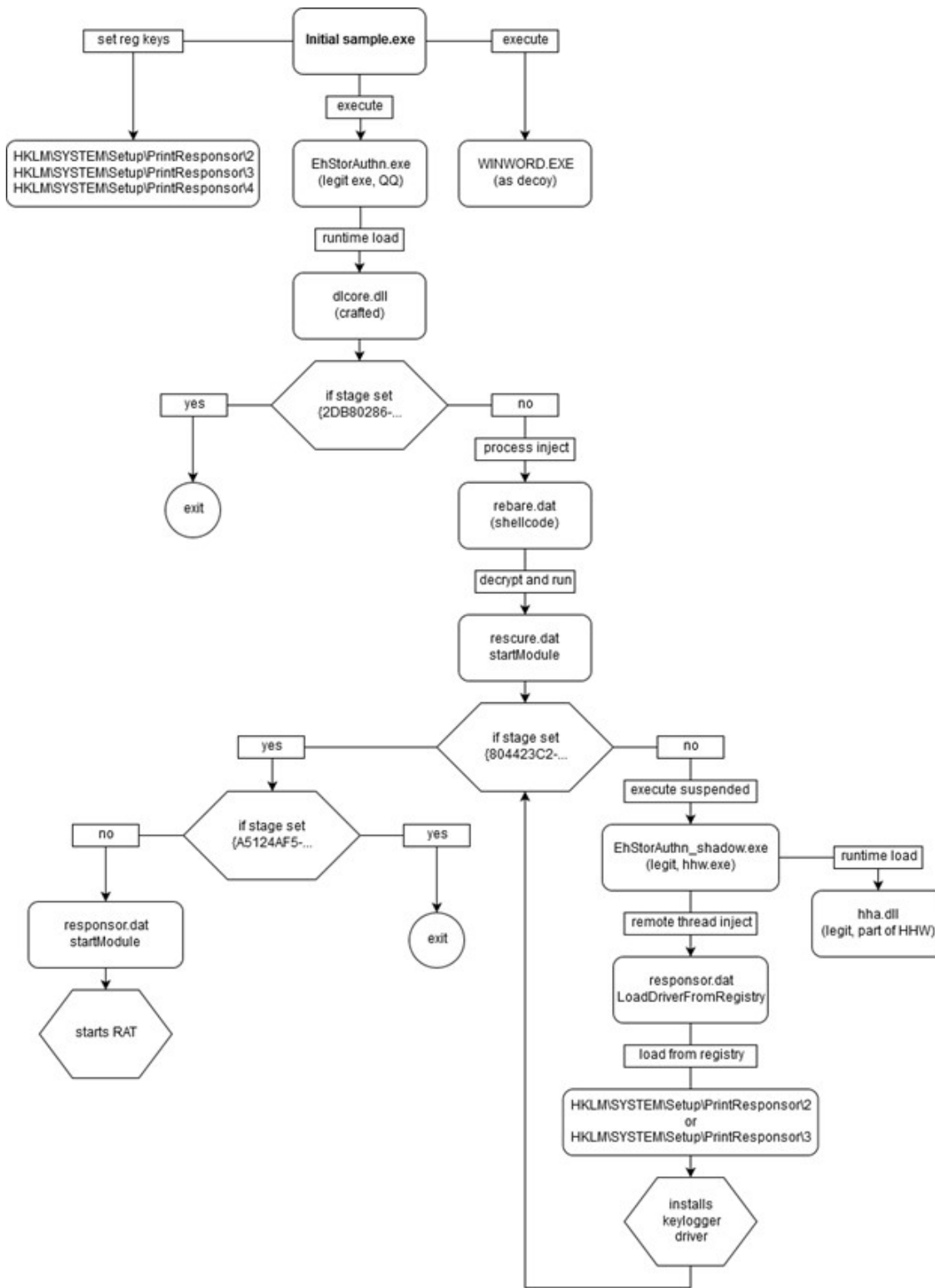
Figure 9 Flowchart of FlowCloud Loader Functionality
