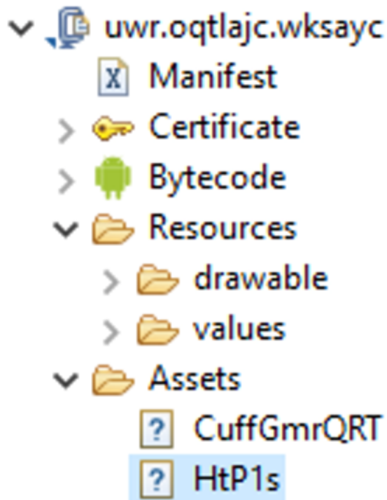
Figure 6. Encrypted executable code in Assets folder
