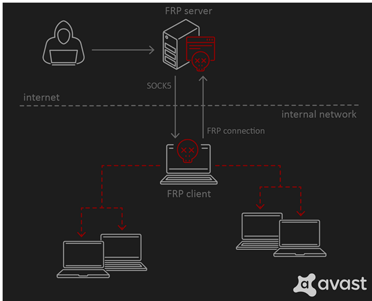
Figure 10: Diagram of FRP tool usage
