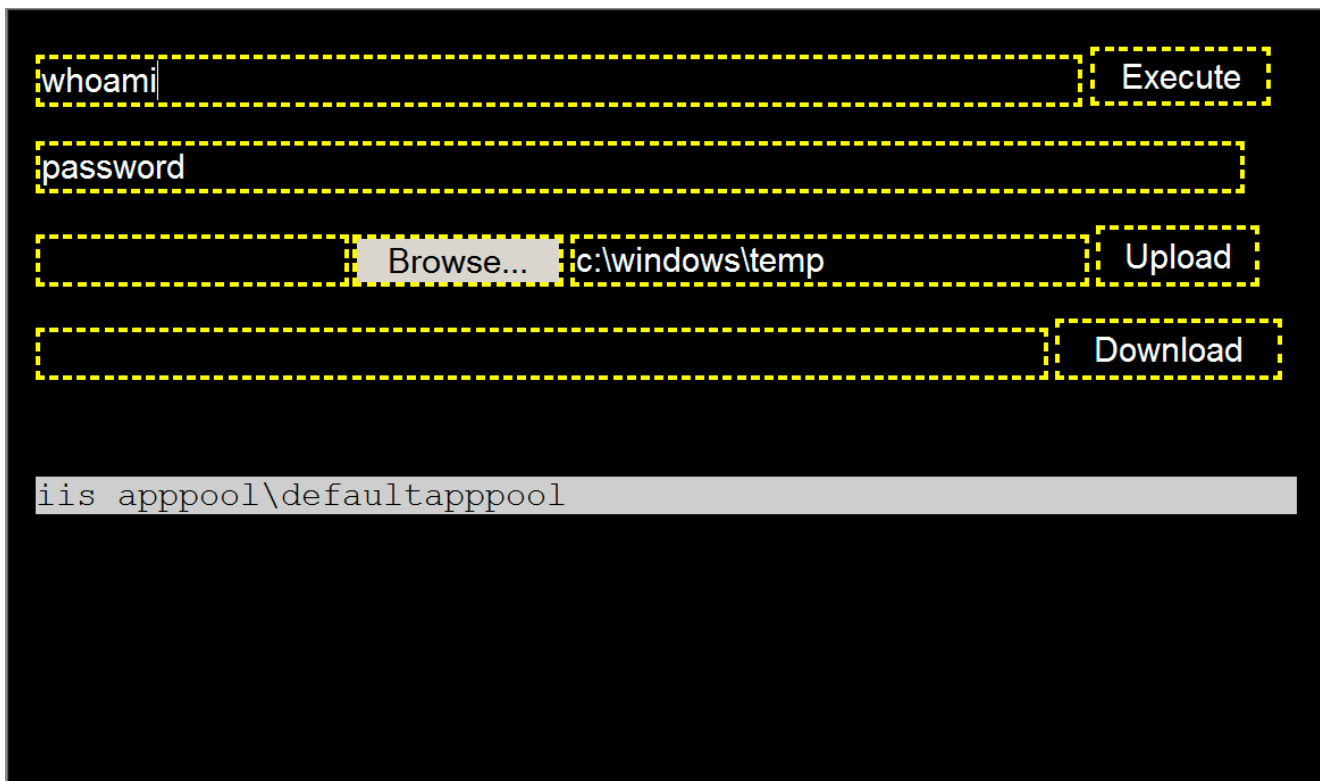
Figure 1. BumbleBee webshell used by xHunt actor to run commands on Microsoft Exchange Server.
