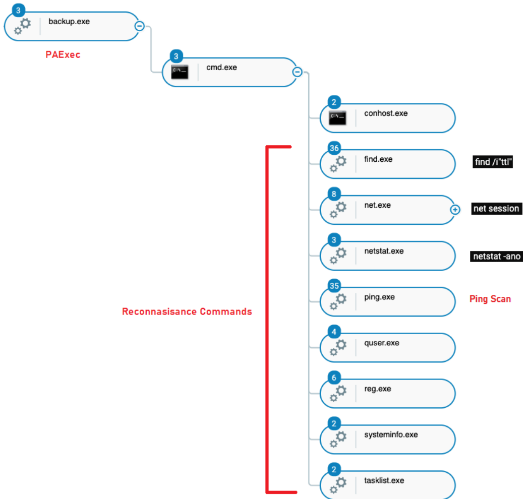
Execution of legitimate tools for reconnaissance and lateral movement as seen in the Cyberreason Defense Platform
