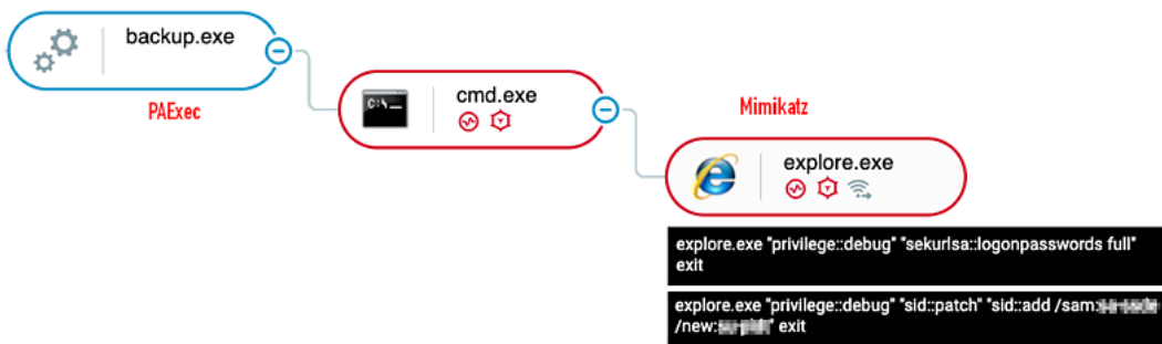
PAExec and Mimikatz execution as seen in the Cybereason Defense Platform
