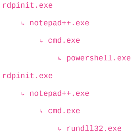
Figure 7: Two FIN7 process event chains
