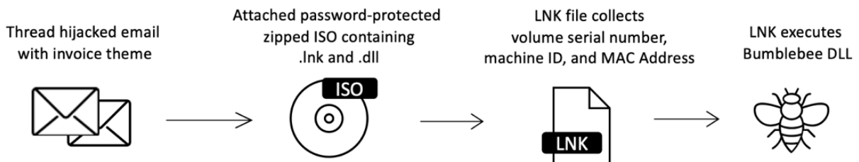
Figure 8: Thread hijacking attack chain leading to Bumblebee
