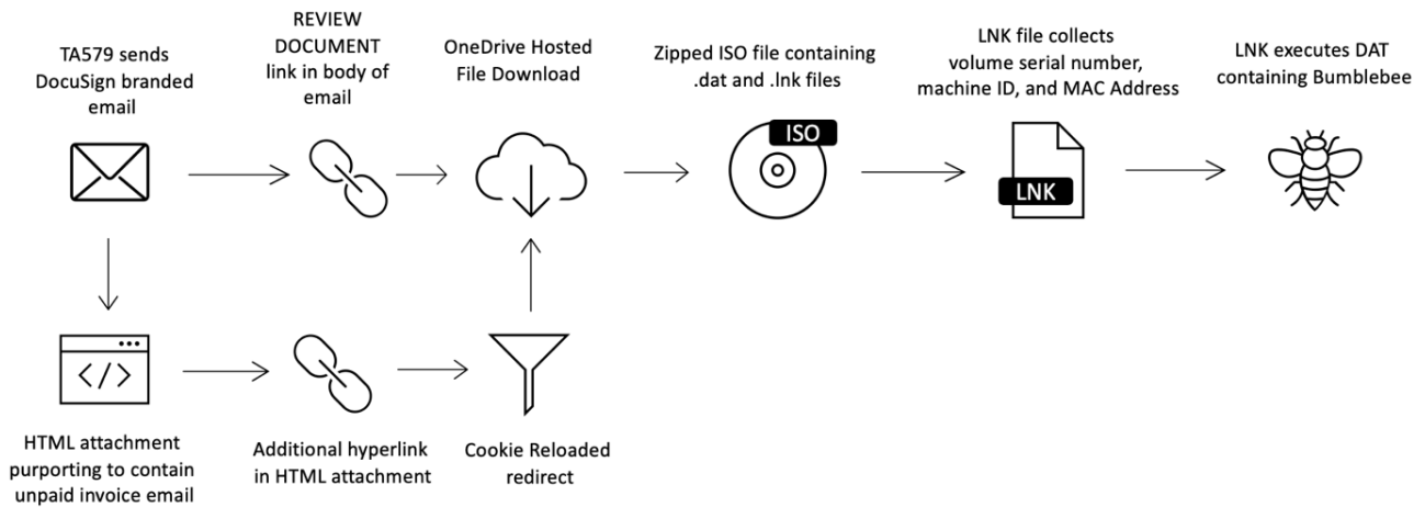
Figure 5: TA579 attack chain leading to Bumblebee
