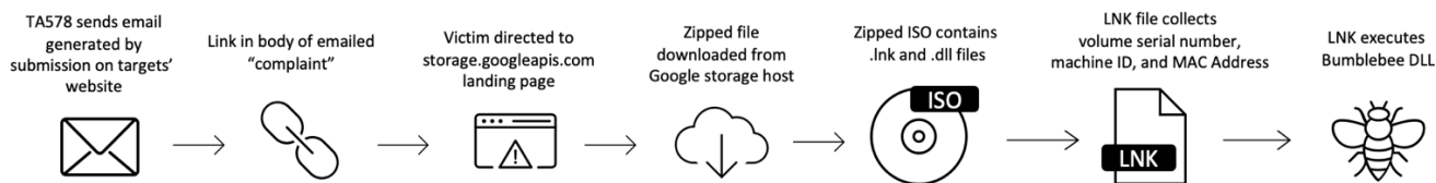
Figure 11: "Contact Form" attack chain leading to Bumblebee
