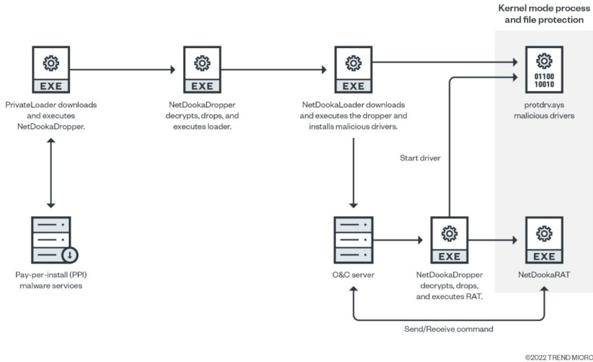
Figure 1. Infection chain of the attack
