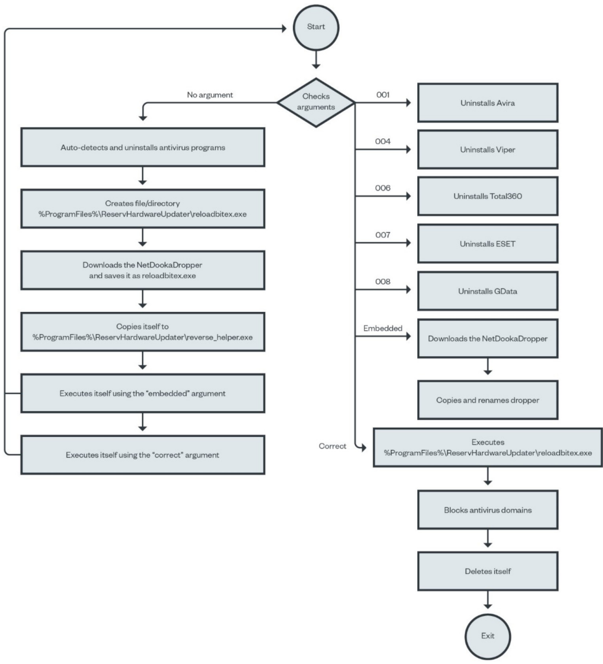
Figure 2. NetDookaLoader flow chart
