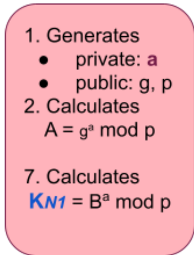
Figure 3. How the basic DHE protocol for key exchange would look between Emilia's computer and the Tor guard node. Note that in practice ECDHE (DHE with elliptic curve crypto) is used with node authentication.
