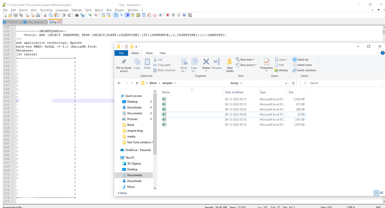
Fig.1 Excel Maldocs
