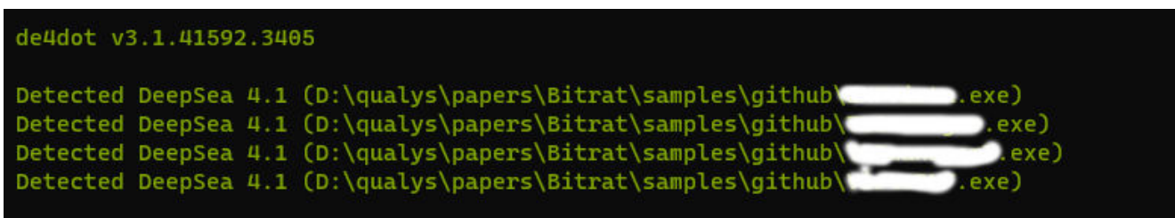
Fig.7 BitRAT obfuscation
