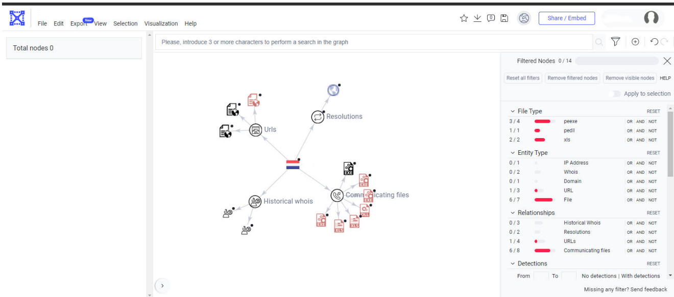
Fig.9 BitRAT C2
