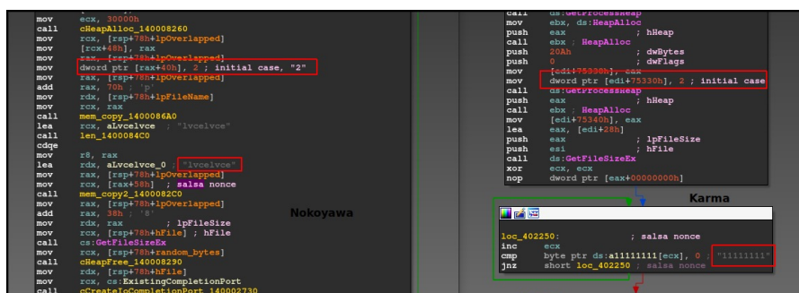
Initial case, encryption thread
