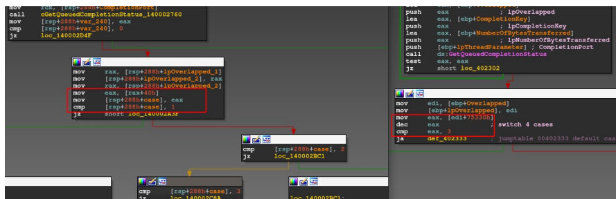
Encryption thread case handler
